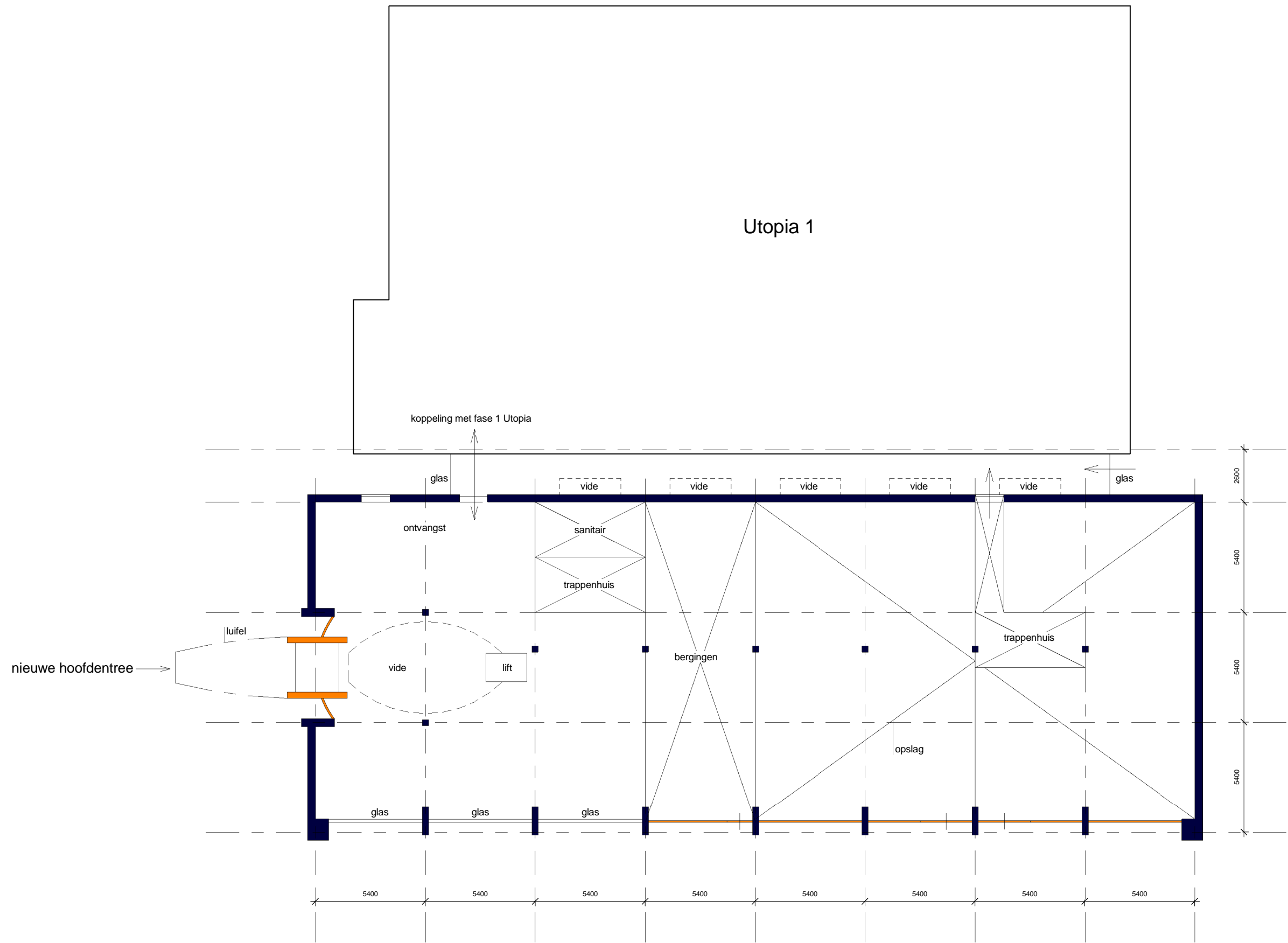
BEGANE GROND bvo ca. 671 m 2
